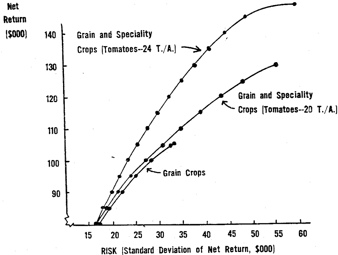
Figure 1. Efficiency Frontiers
